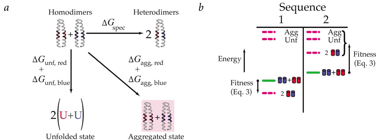
Fig. 2 Positive and negative design states. a , Schematic representation of competing states included in the design calculations targeting the homodimer conformation. Competing states are included to enforce homosppecificity (upper right), solubility (lower right) and stability (lower left). The aggregated state is modeled as the target conformation embedded in a medium with a dielectric constant of 65. Each sequence considered by the genetic algorithm is subjected to conformational optimization in each of the four states. The fitness score for a given sequence is the transfer free energy from the target state (homodimer) to the ensemble of competing states (heterodimers, aggregated state and unfolded state). \Delta G_{\text{spec}} and \Delta G_{\text{unf}} are transfer free energies between states and can be measured experimentally. b , Energy diagram for two protein sequences in different conformational or associative states. A solid green line indicates the energy of the target state, the coiled-coil homodimers. The dashed magenta lines indicate the energies of competing states, including the unfolded protein, aggregated protein and the coiled-coil heterodimers. Sequence 1 minimizes the energy of the target state and would be incorrectly selected by the single-state design algorithm. The single-state design algorithm cannot recognize that the heterodimers are more stable than the homodimers because stabilities are computed only for the target state. The multi-state algorithm would correctly select sequence 2, because its transfer free energy from the target state to the ensemble of competing states is more positive than for sequence 1 (Eq. 3).
