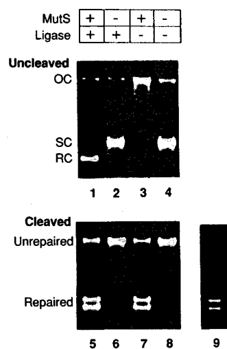
Fig. 2. Requirement for DNA ligase in mismatch correction. Hemimethylated G-T heteroduplex DNA [Fig. 1, 0.6 \mu g, d(GATC) methylation on the complementary DNA strand] was subjected to mismatch repair under reconstituted conditions in a 60- \mu l reaction (Table 3, closed circular heteroduplex), or in 20- \mu l reactions (0.2 \mu g of DNA) lacking MutS protein or ligase, or lacking both activities. A portion of each reaction (0.1 \mu g of DNA) was treated with EDTA (10 mM final concentration) and subjected to agarose gel electrophoresis in the presence of ethidium bromide (1.5 \mu g/ml; top panel, lanes 1 to 4). Positions are indicated for the unreacted, supercoiled substrate (SC), open circles containing a strand break (OC) and covalently closed, relaxed circular
